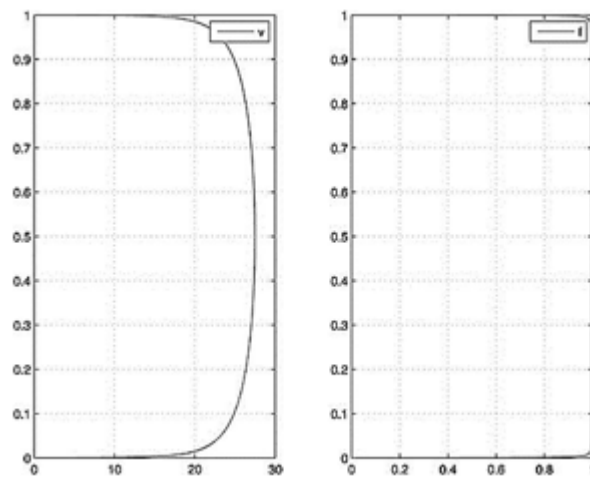
Рис. 5. Re_+ = 10^4
